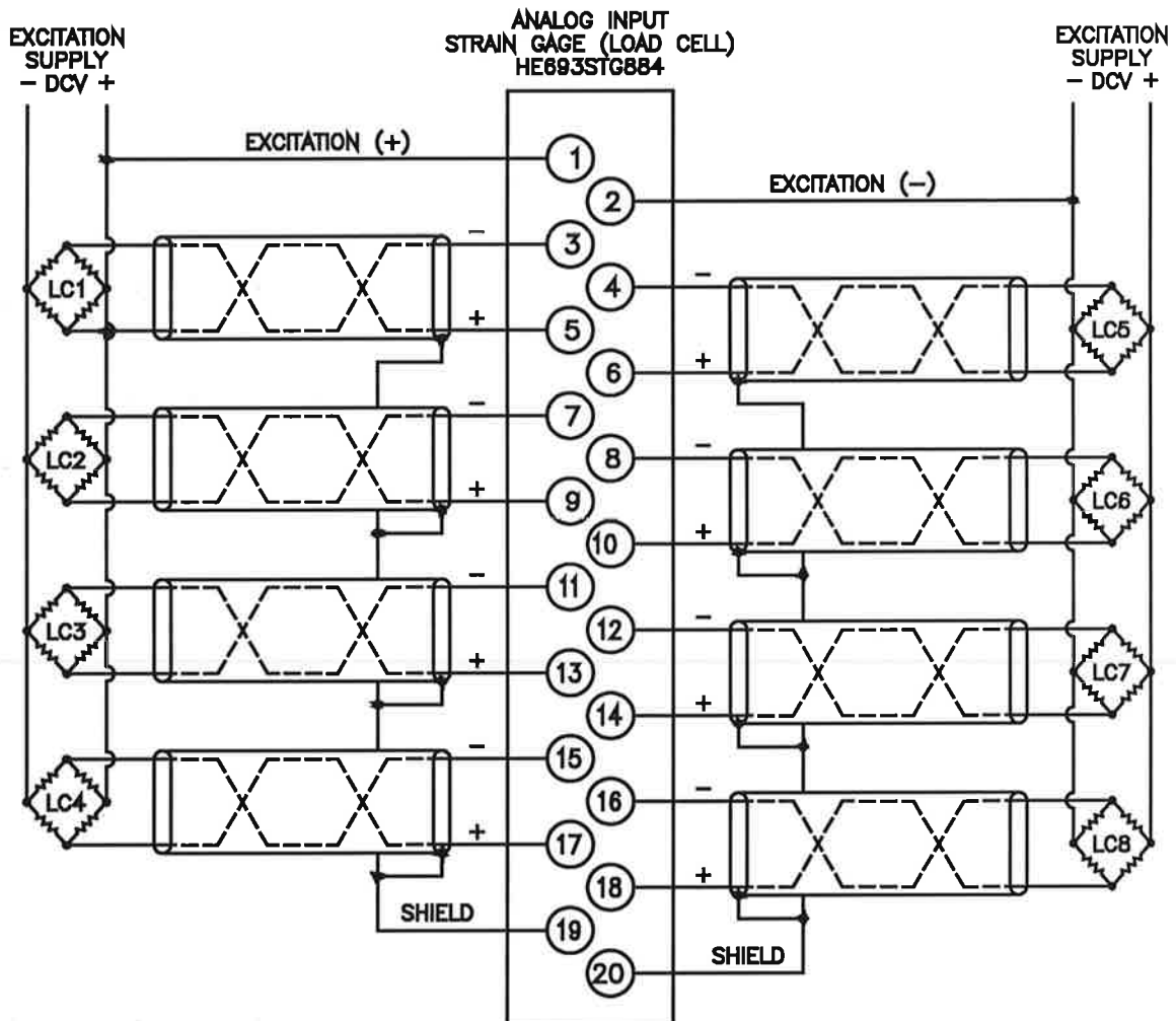
Figure 3.1 – Wiring Diagram
