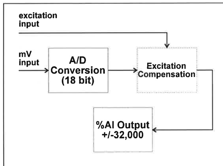
Figure 4.2 Excitation Compensation
