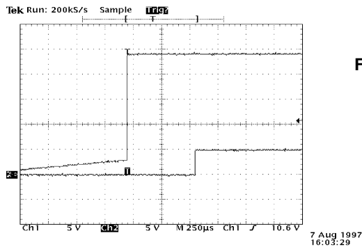
Figure B.2 - Case Example: IC693MDL655 Digital Input Module Wave Forms
