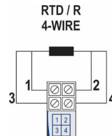
Fig. 9 – Transmitter electrical connections (Pt100 4-wire)
