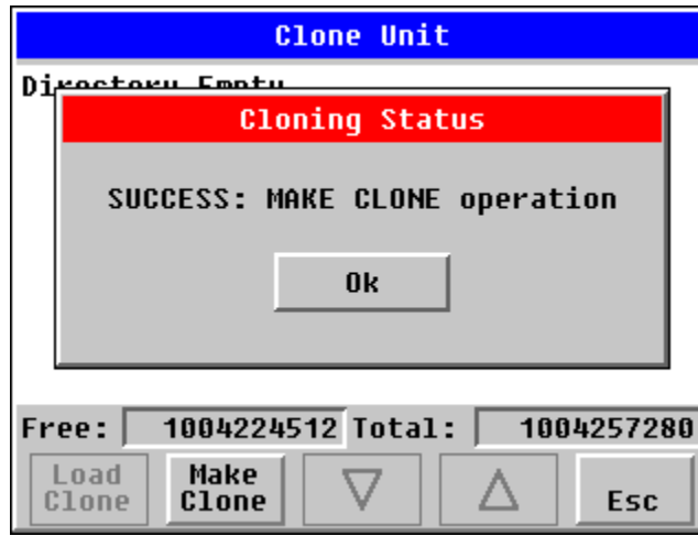
Figure 5 - Cloning Status
