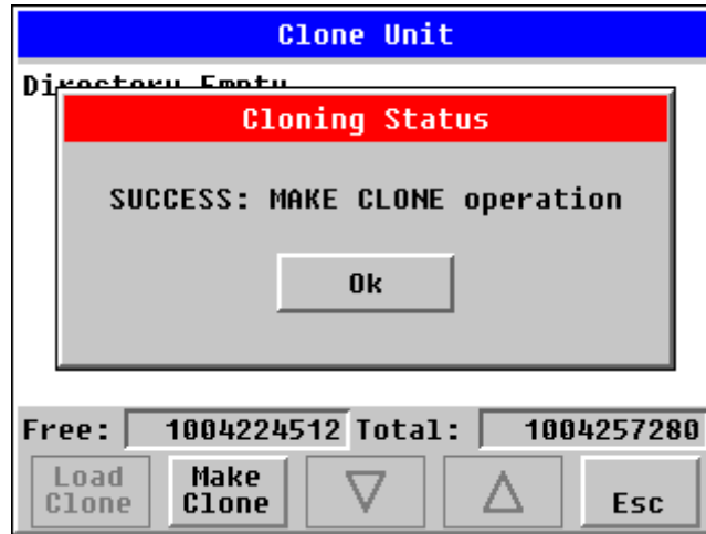
Figure 5 - Cloning Status
