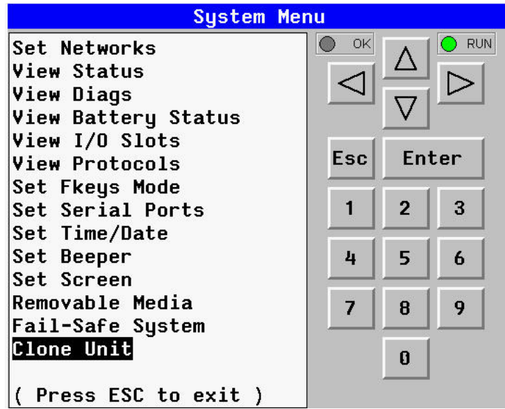
Figure 1 - System Menu
