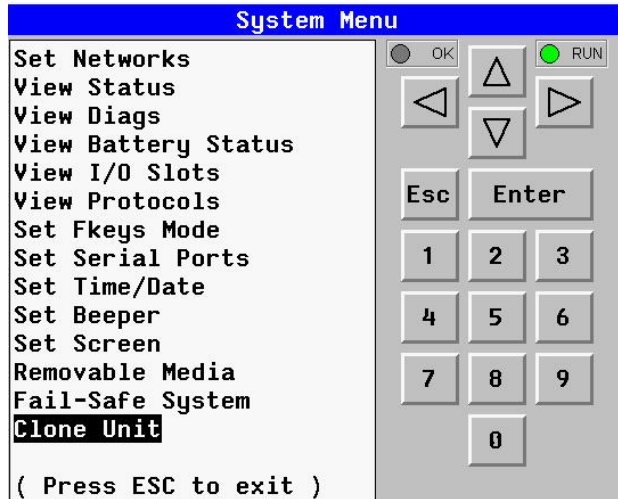
Figure 6 - System Menu
