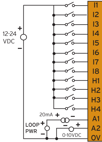
20mA Analog In - Not Self Powered
