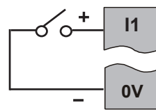
Negative Logic In
