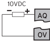
0 - 10V Analog Out
