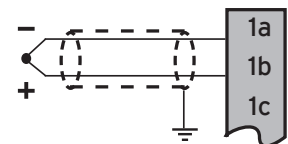
Thermocouple In
