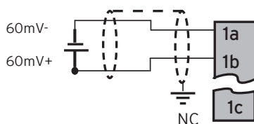
mV In
