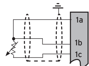
RTD In
