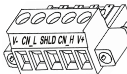
CAN Pin Assignments
